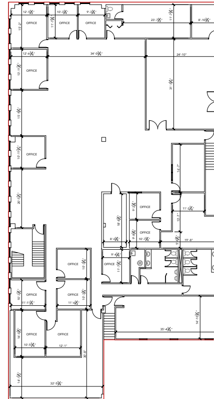
Second Floor Office Plan
