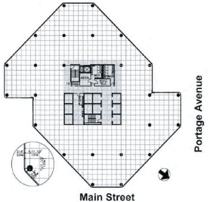
Low-Rise (Floors 1-16)
